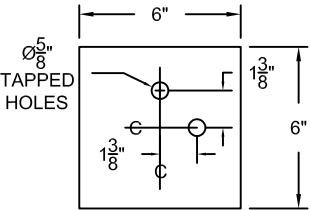
TOP PLATE DETAIL
