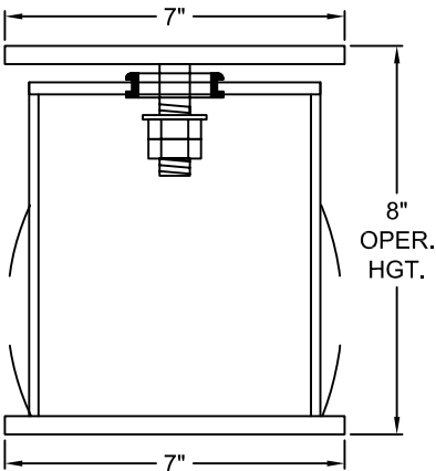
End View
