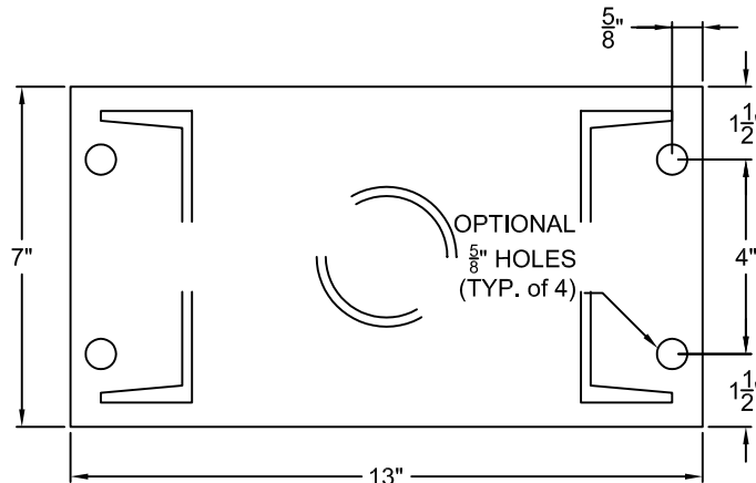
Base Plate
