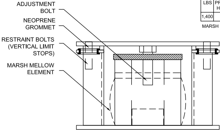
Side View
